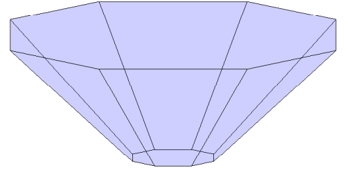
Figura 3.18: politopo \Omega
